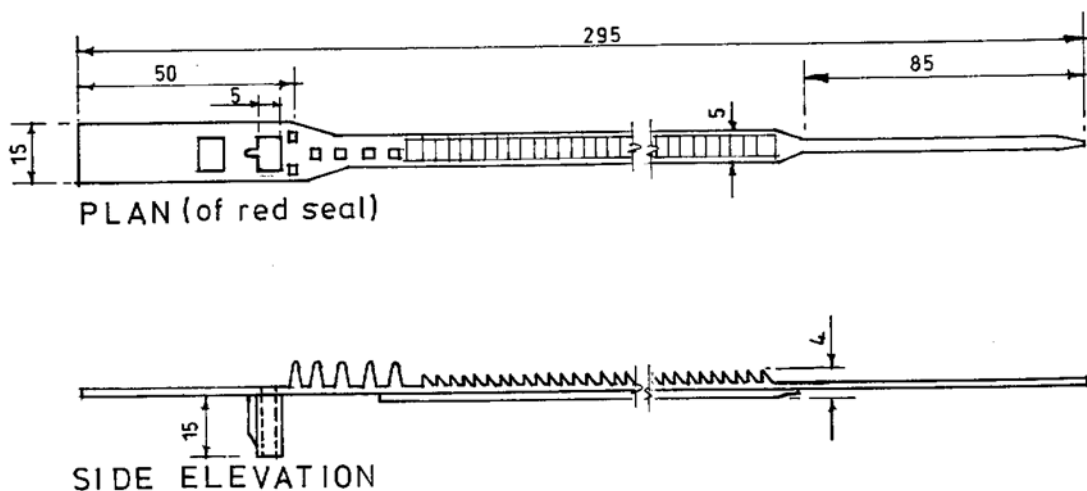
Figure 1 — Typical dimensions of a security seal
