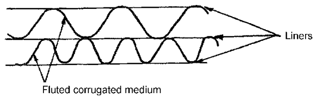
Fig. 2 — Double-wall corrugated fibreboard
